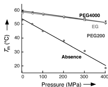
Figure 2: Dependencies of T m for G-quadruplex DNA on pressure in the presence of EG (□), PEG200 (◇), PEG4000 (x), and in the absence of cosolute (○).
